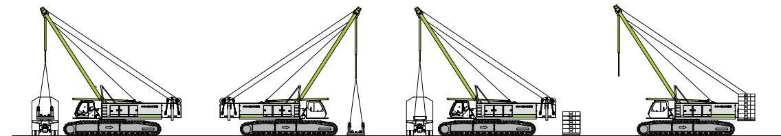
Unloading and assembly of rear counterweight
